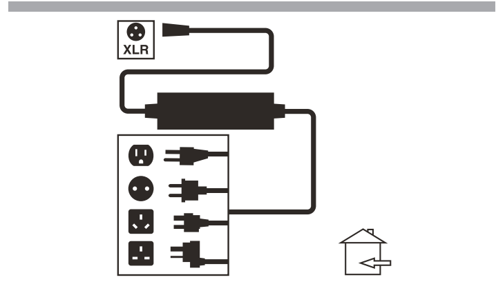
Figure 18. Battery Charger
