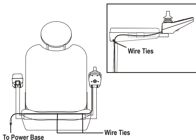
Figure 7. Controller Harness Routing on a Contour Seat
