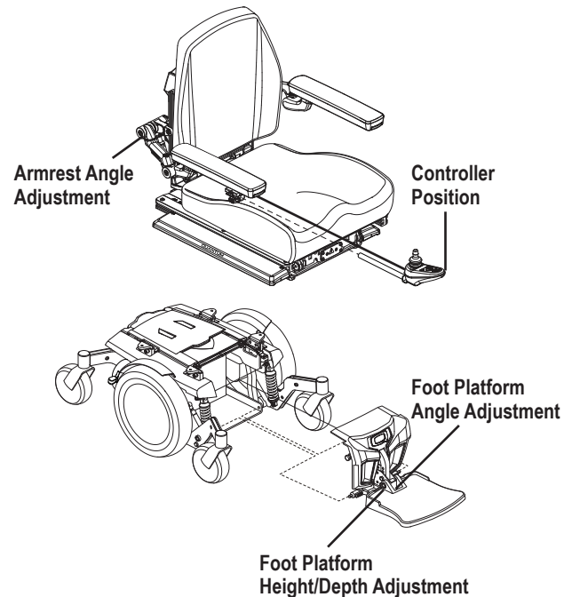
Figure 4. Assembly View
