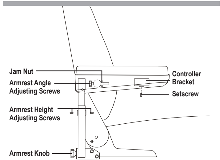
Figure 14. Seatback/Armrest Adjustment
