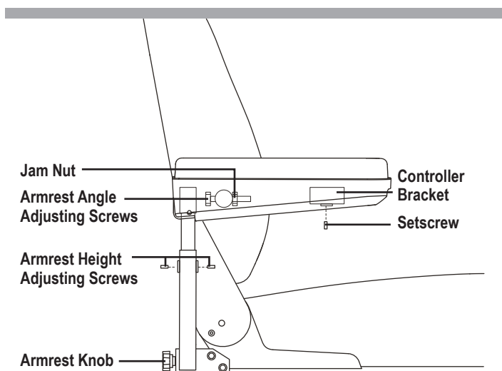
Figure 16. Seatback/Armrest Adjustment
