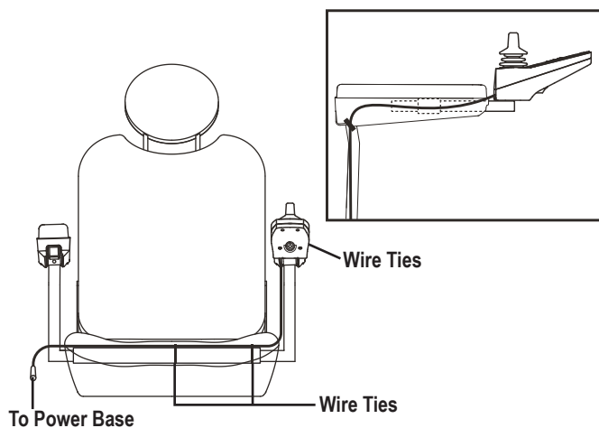
Figure 8. Controller Harness Routing on a Contour Seat
